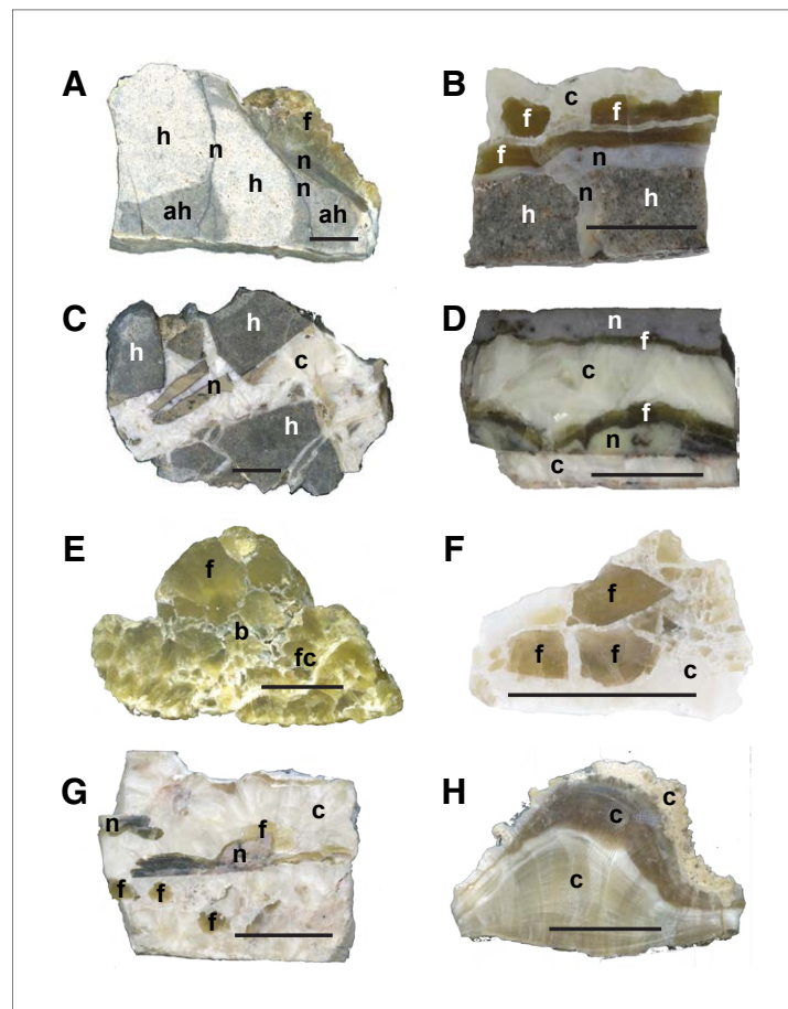
Figure 2. Visible light images of the samples from the fracture. (A) Host rock with small veins that are filled by nacrite and capped by fluorite. (B) Fractured host rhyolite with nacrite between fragments and on surfaces followed by fluorite, which is brecciated and cemented by calcite. (C) Brecciated host rhyolite and nacrite that is cemented by calcite. (D) Layered vein material with the calcite on the bottom appearing to be the surface upon which nacrite followed by fluorite followed by calcite grew. These minerals appear to come from the top and bottom. (E) Brecciated green fluorite with calcite filling between some fragments. (F) Brecciated fluorite with calcite cement. (G) Breccia with nacrite and fluorite clasts. (H) Two generations of calcite. The white to amber calcite is highly enriched in rare-earth elements (REEs). The brown calcite is low in REE but has high U-Pb ratios. Labels are: h—host; ah—altered host; n—nacrite; f—fluorite; fc—fluorite with calcite; c—calcite; b—brecciated zone. Not visible here is the yttrium and heavy rare-earth element (YHREE) carbonate that lines the breccia clasts and occurs between fluorite and calcite. Scale bars are all 1 cm.
